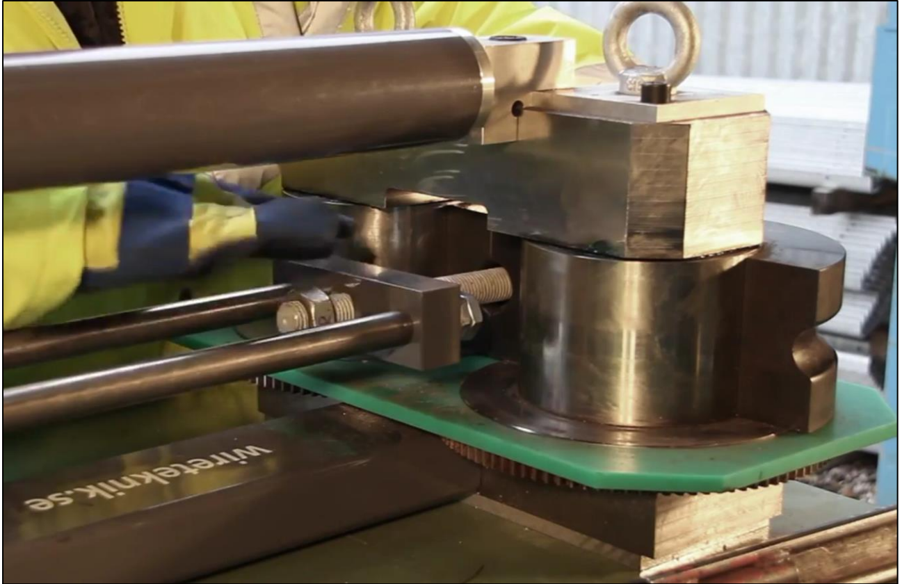
Figure 5: Fitting attachment to pulling block
