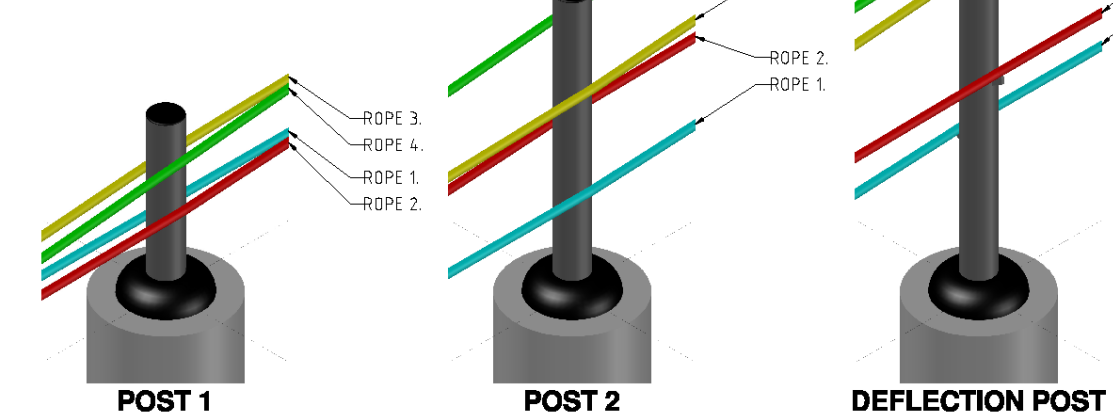
DETAIL A
