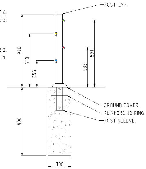
DEFLECTION POST (ELEVATION)
