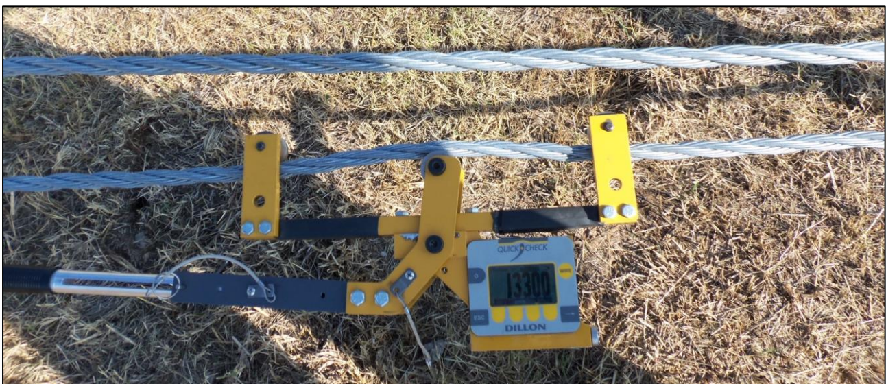
Figure 16: Tension Meter Attachment
