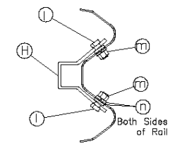
SECTION C-C Anchor Bracket
