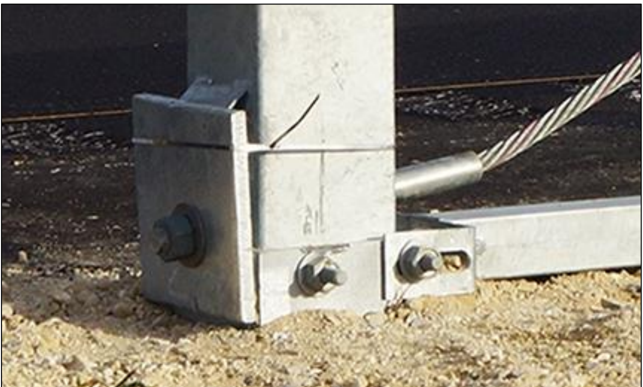
Post 1 Connection Detail
