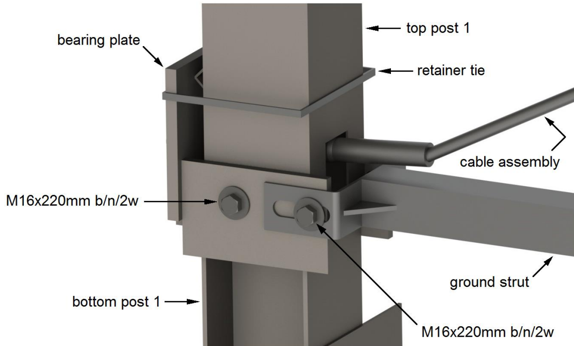
Figure 8: Post 1 Connection Detail
