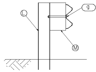
SECTION B-B Posts #3 thru #8
