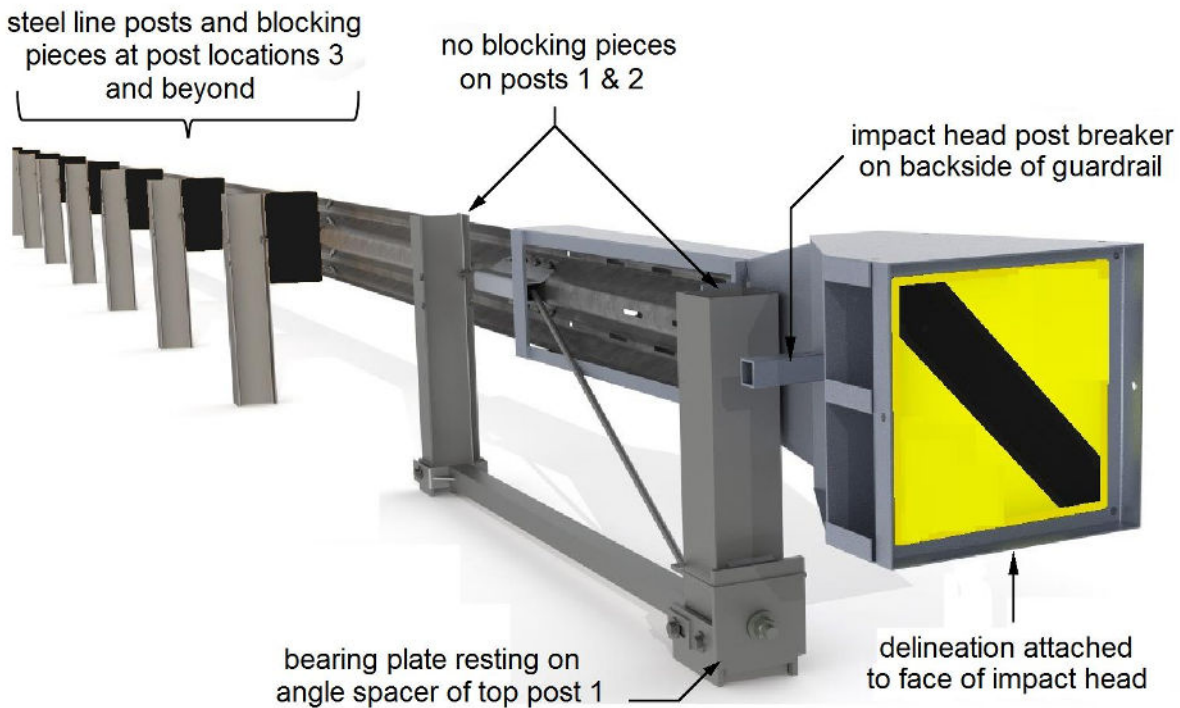
Figure 10: Cable Assembly and Impact Head Assembly Detail
