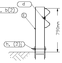
SECTION A-A Post #2
