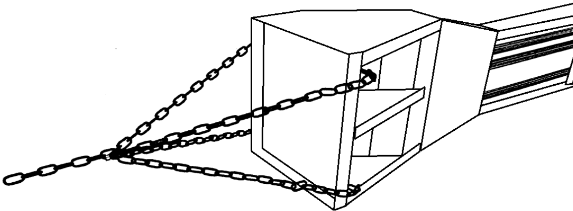
Figure 12: Attachment of Chains for Removal of Impact Head
