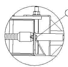
Impact Head Connection Detail
