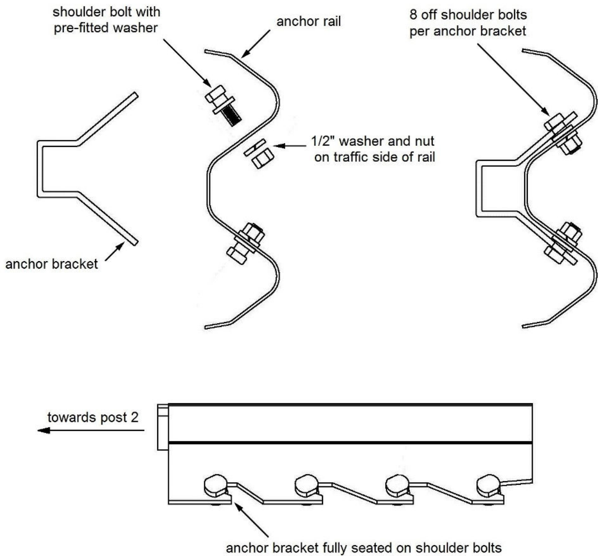
Figure 9: Attachment of Cable Anchor Bracket
