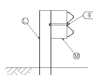
SECTION B-B Posts #3 thru #5
