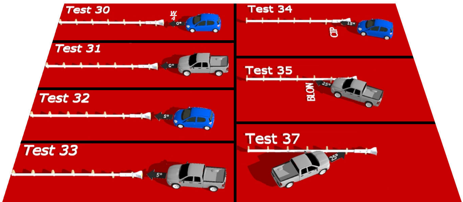
Figure 1: MASH End Terminal Crash Test Evaluation
