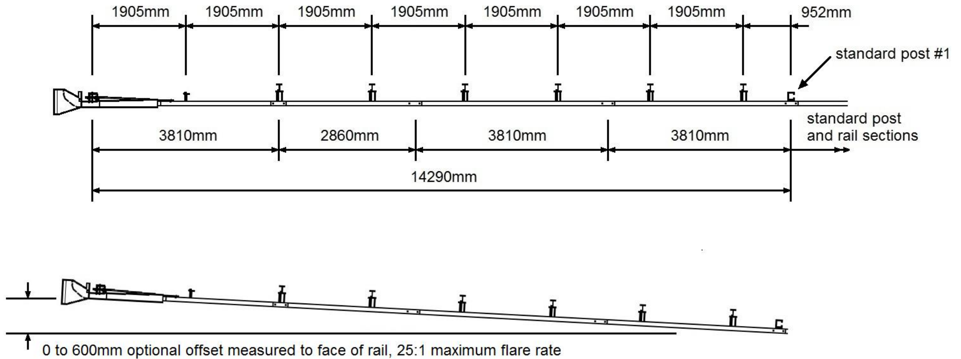
Figure 3: MSKT Set-Out (TL3)
